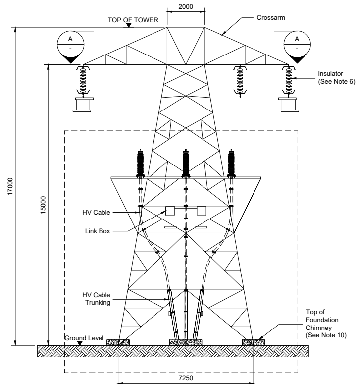
Front Elevation (Rear Platform Removed for Clarity)
