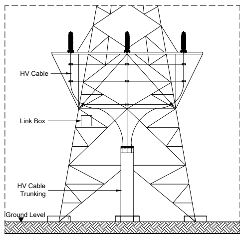
Variation on Trunking Front Elevation (See Note 7)
