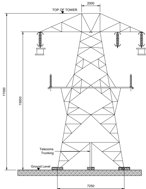
Rear Elevation (Front Platform Removed for Clarity)
